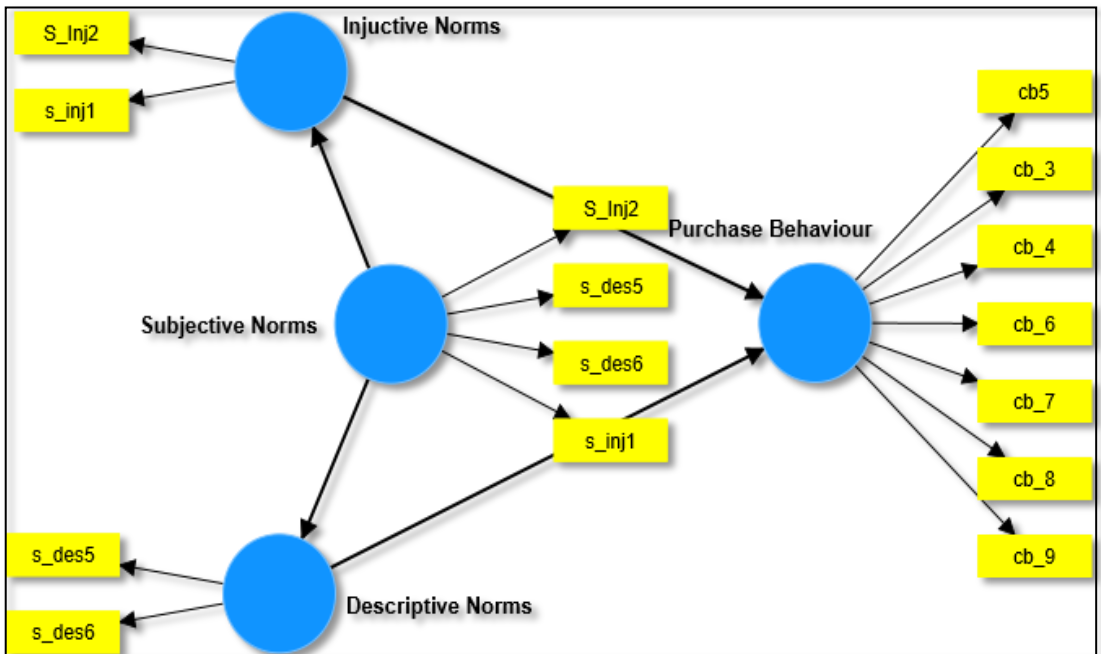
Figure 1. Measurements Model
